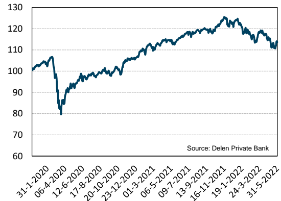
NAV evolution of HU ONE Dynamic C Cap* since launch
